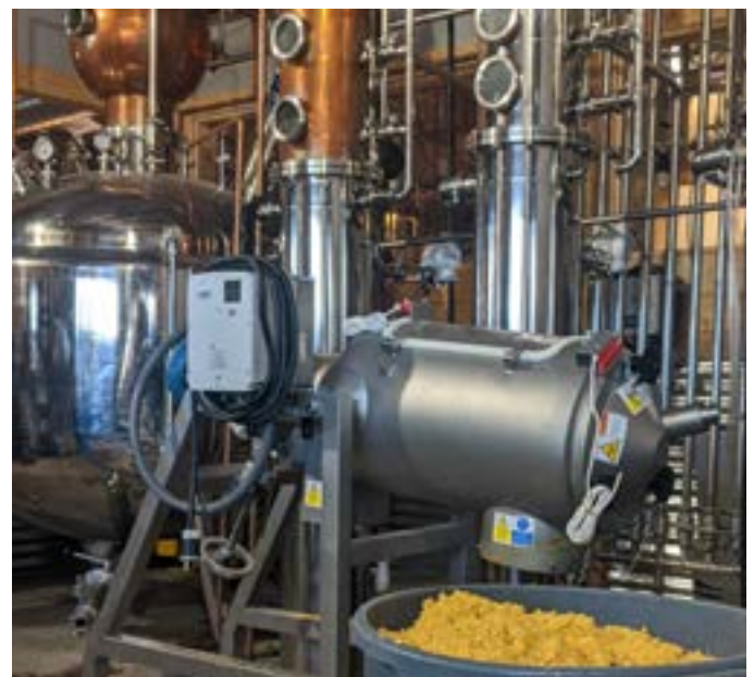
Figure 1. The Liquid Solid Separator™ is installed at Blue Valley Spirits to remove spent grains from ethanol
